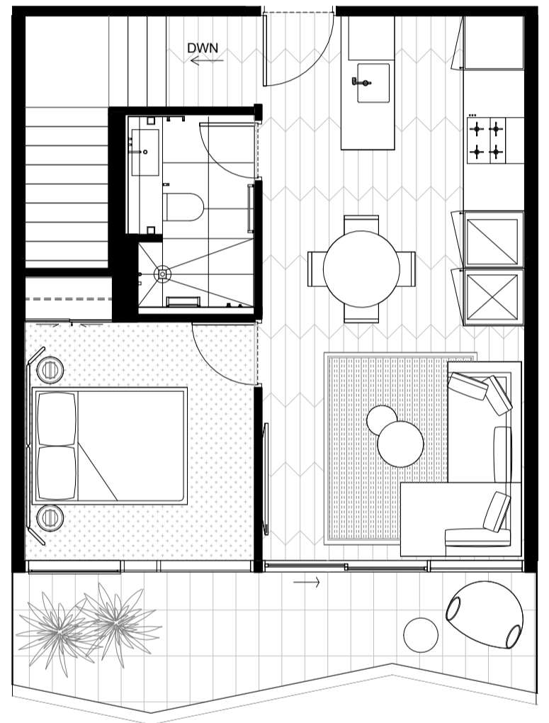
LEVEL 01
