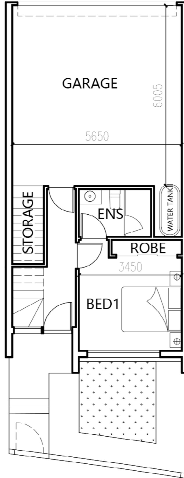
Ground Floor
