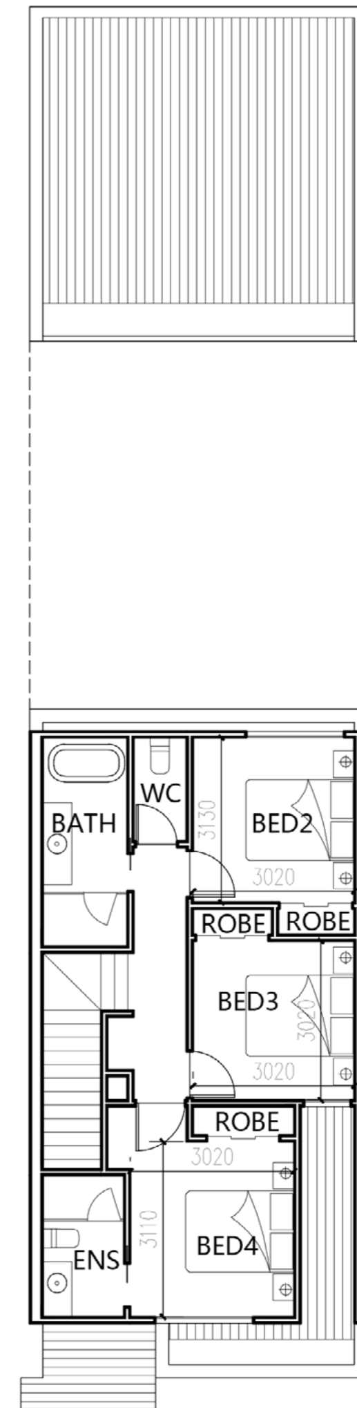
First Floor
